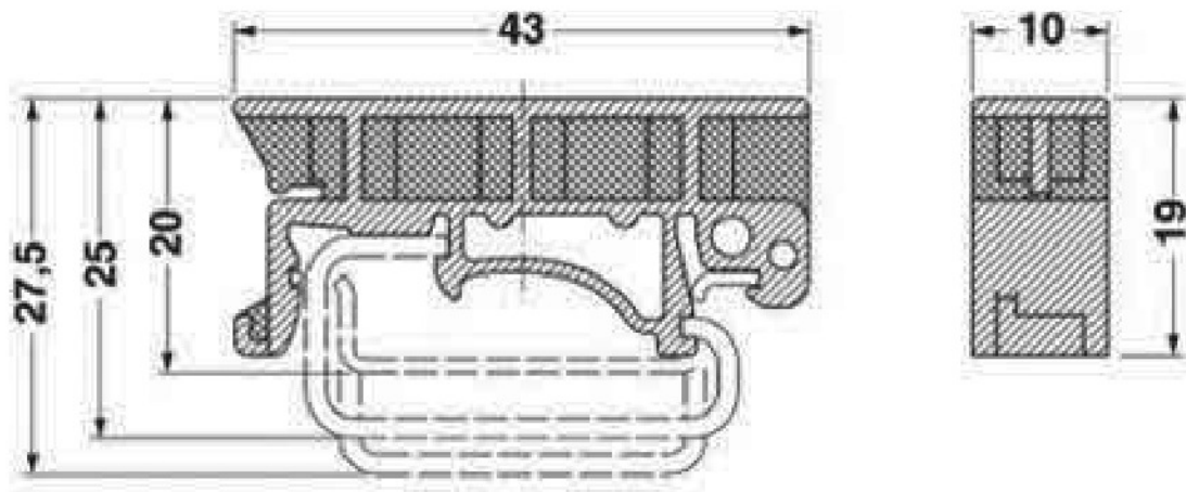
Dimensioned drawing
